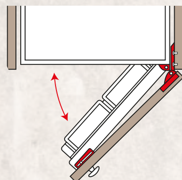
Additional space is required on the inner side of the cabinet to make way for the door hinge.
